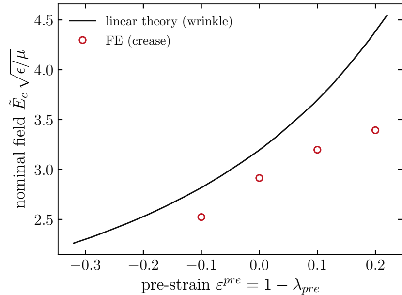
Nominal critical field, \bar{\gamma} = 2
