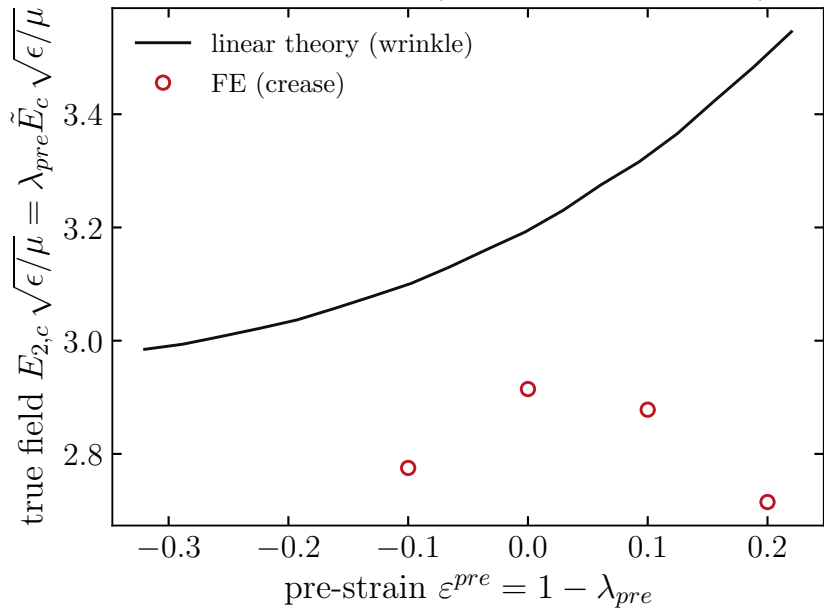
True critical field (nearly \lambda -independent)
