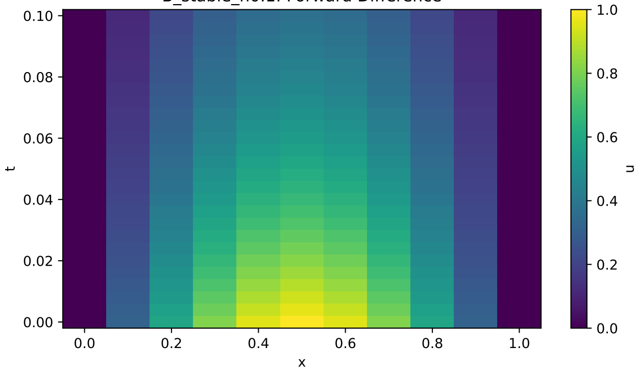
B_stable_h0.1: Forward Difference
