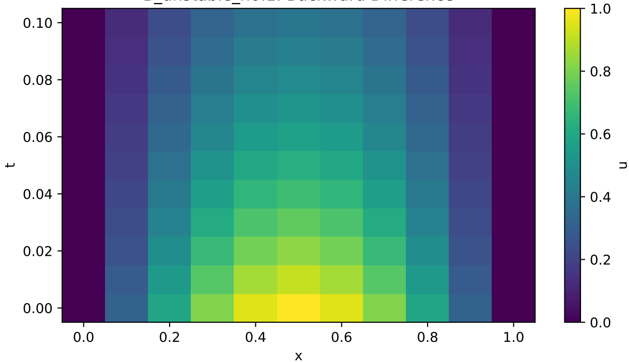
B_unstable_h0.1: Backward Difference
