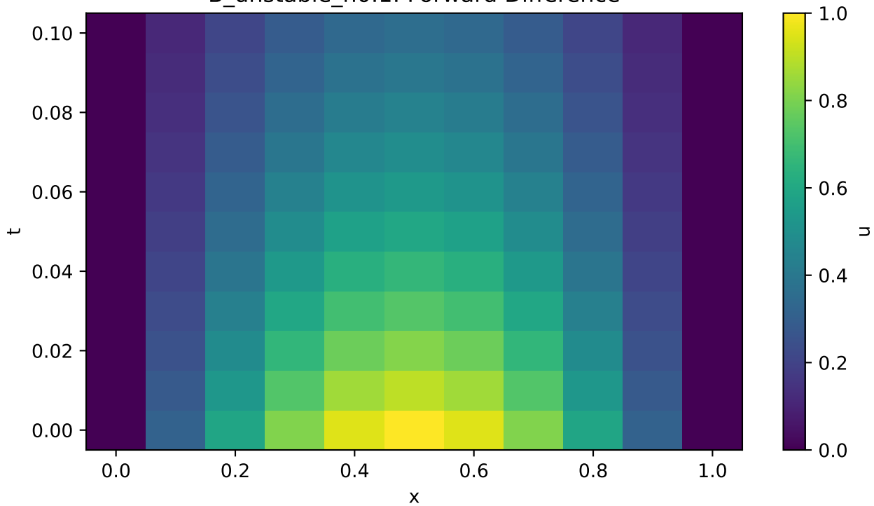
B_unstable_h0.1: Forward Difference
