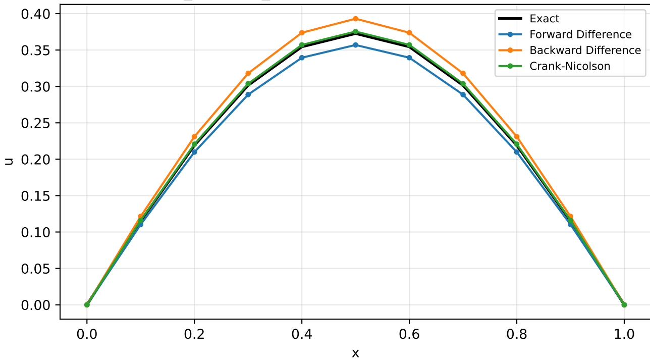
B_unstable_h0.1: final time t=0.1 , \lambda=1
