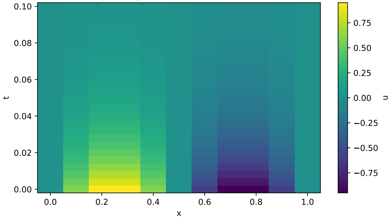
C2_stable_h0.1: Backward Difference
