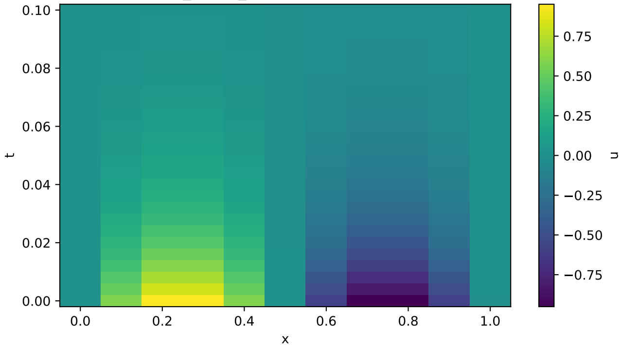
C2_stable_h0.1: Crank-Nicolson
