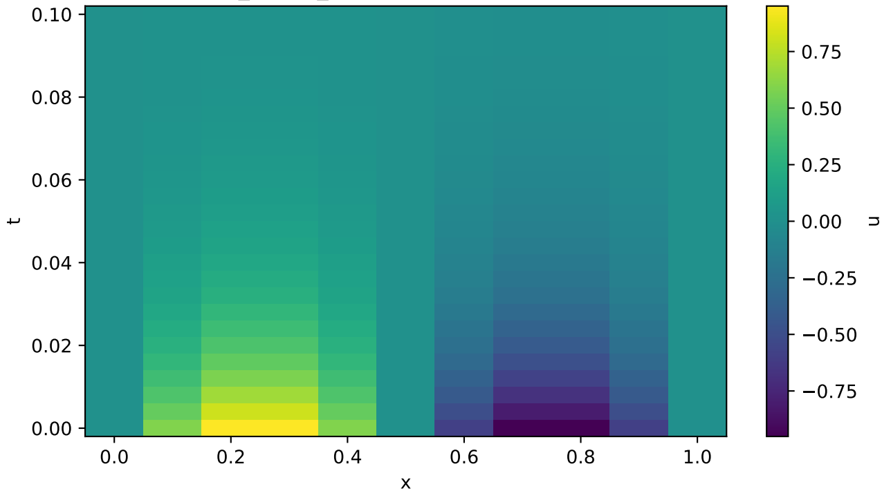
C2_stable_h0.1: Forward Difference
