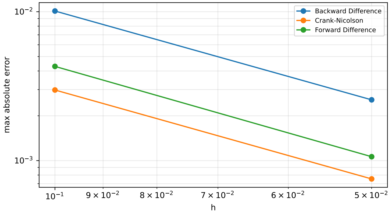
B: max error vs mesh size
