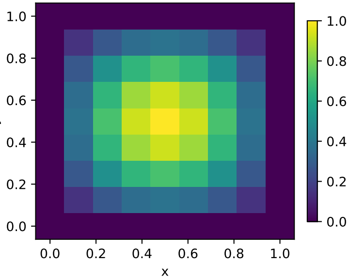
Exact
