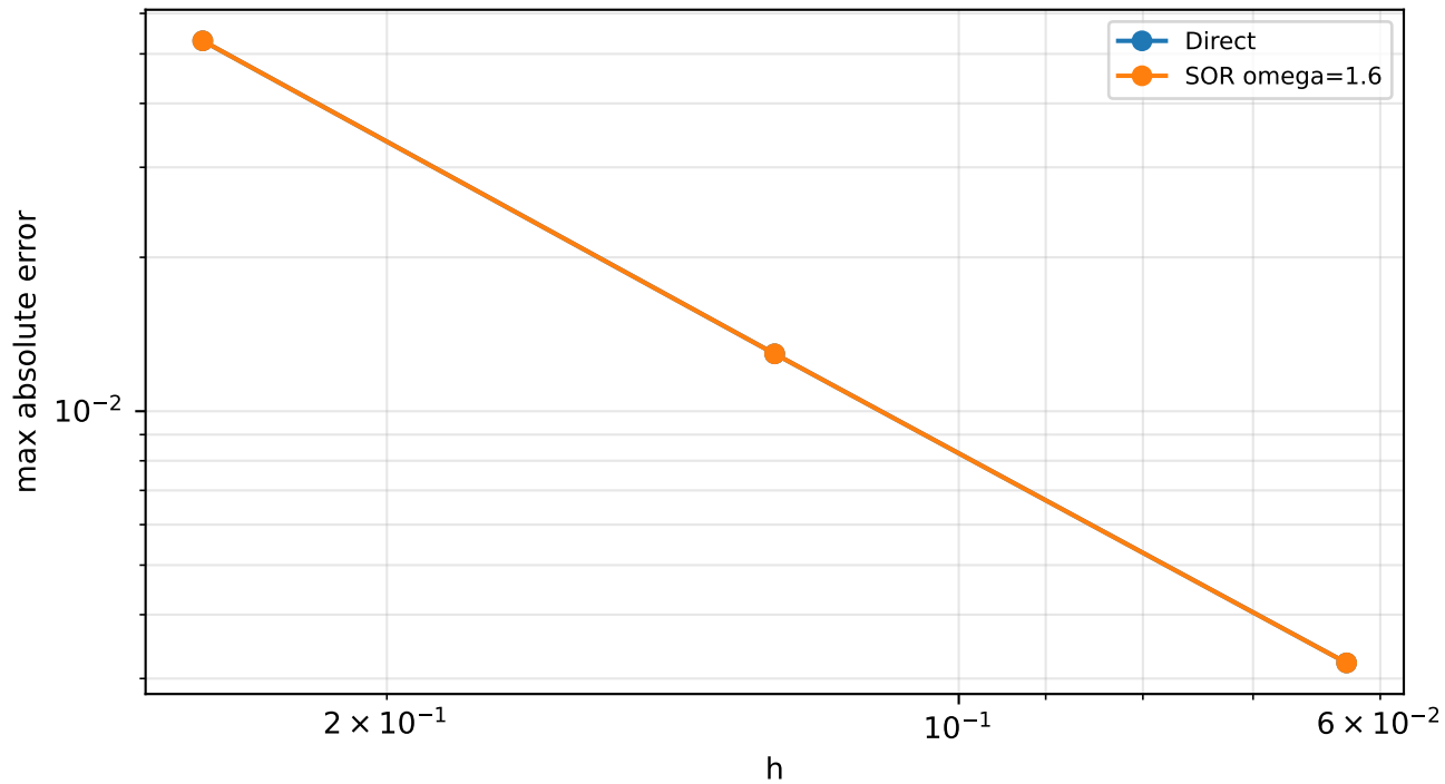
C1: max error vs mesh size
