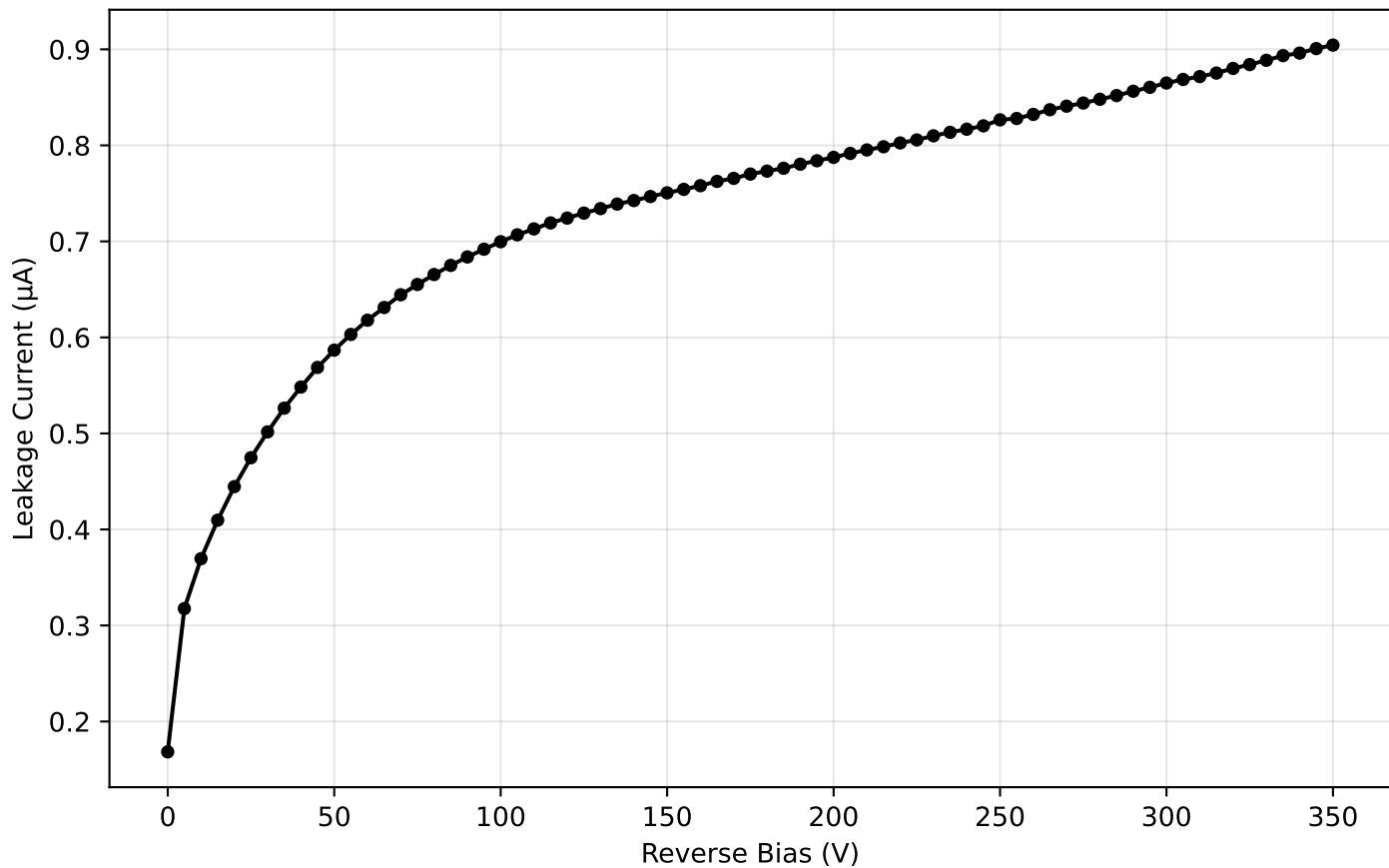
IV Curve: H-1203
