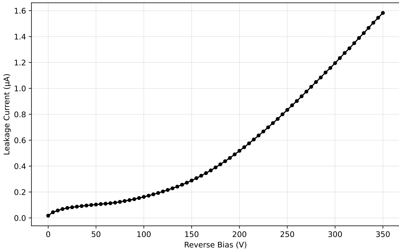
IV Curve: P-1009
