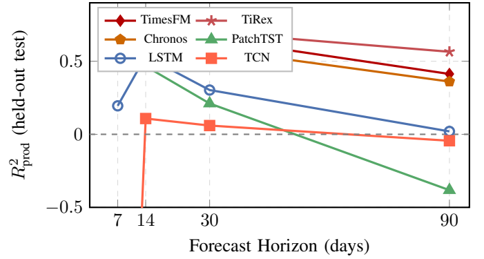
Fig. 3: R^2_{\text{prod}} vs. forecast horizon (Ganymede, held-out test, multi-well). Foundation models (top 3 curves) consistently outperform trained models. DeepONet omitted ( R^2 < -5 ). TCN omitted from y-axis range due to R^2_{\text{prod}} = -4.51 at h=7 . Dashed line: R^2=0 (naive baseline).
