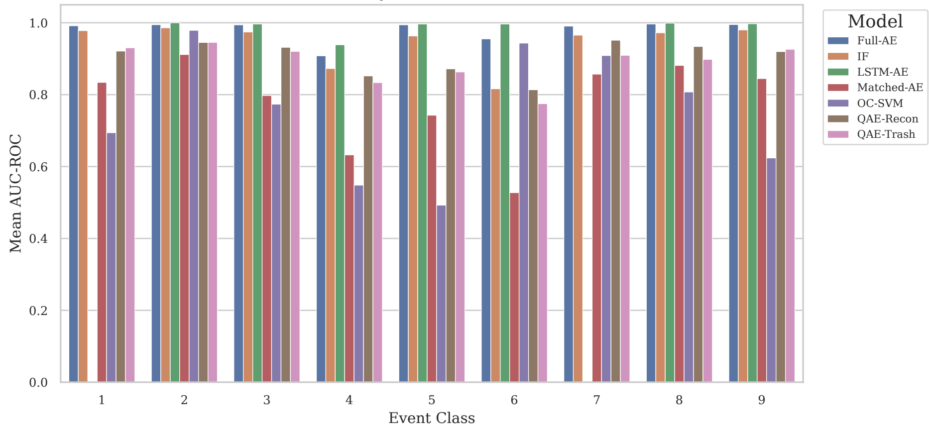
AUC-ROC by Model and Event Class
