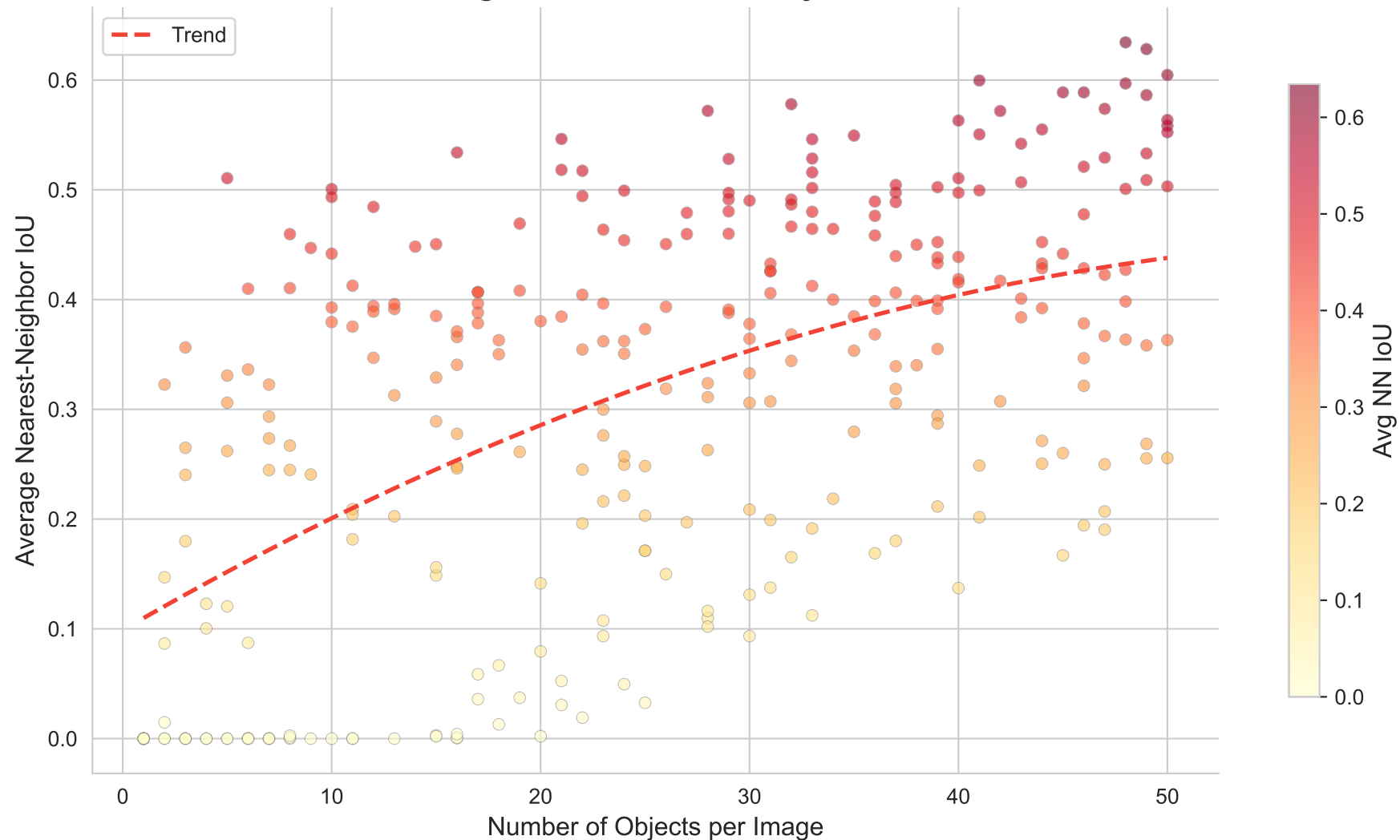
Figure 3: Occlusion Analysis
