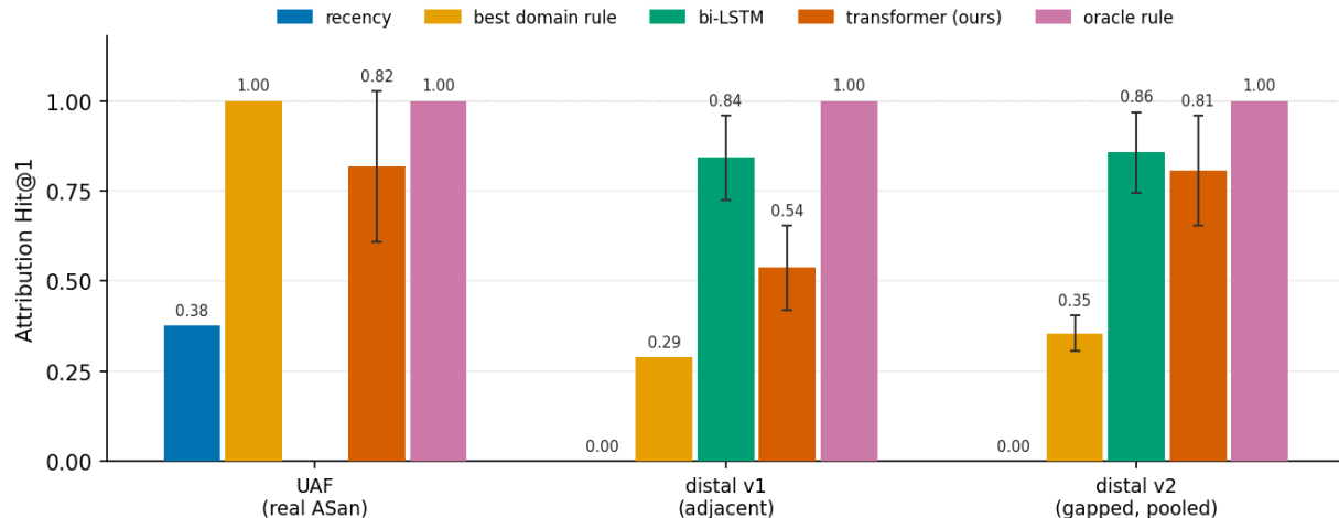
Figure 1: Attribution Hit@1 by corpus and method. The learned transformer sits below the oracle rule on every corpus and at or below a generic bi-LSTM; it clears the recency-family baselines but never the oracle or the LSTM. Transformer bars use object bias 4; the UAF and v2 transformer bars and the v2 same-object-write bar are pooled over three corpus realizations, the rest are a single realization. Error bars are \pm population standard deviation over five model-init seeds; deterministic rules have none. Produced by fig1_summary.py .
