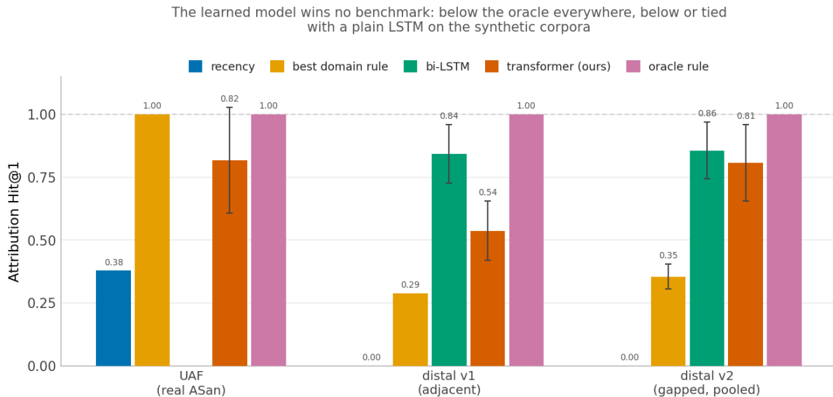
Figure 1. Attribution Hit@1 by corpus and method. The learned transformer sits below the oracle rule on every corpus and at or below a generic bi-LSTM; it clears the recency-family baselines but never the oracle or the LSTM. Transformer bars use object bias 4; the UAF and v2 transformer bars and the v2 same-object-write bar are pooled over three corpus realizations, the rest are a single realization. Error bars are \pm population standard deviation over five model-init seeds; deterministic rules have none. Produced by fig1_summary.py .
