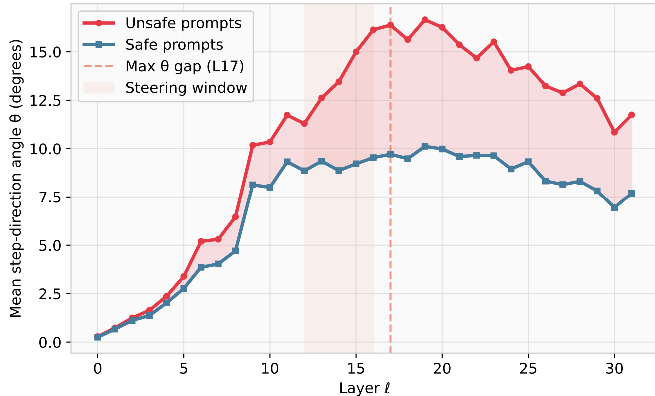
(a) IT→DPO Step Angle — Divergence peaks at L17
