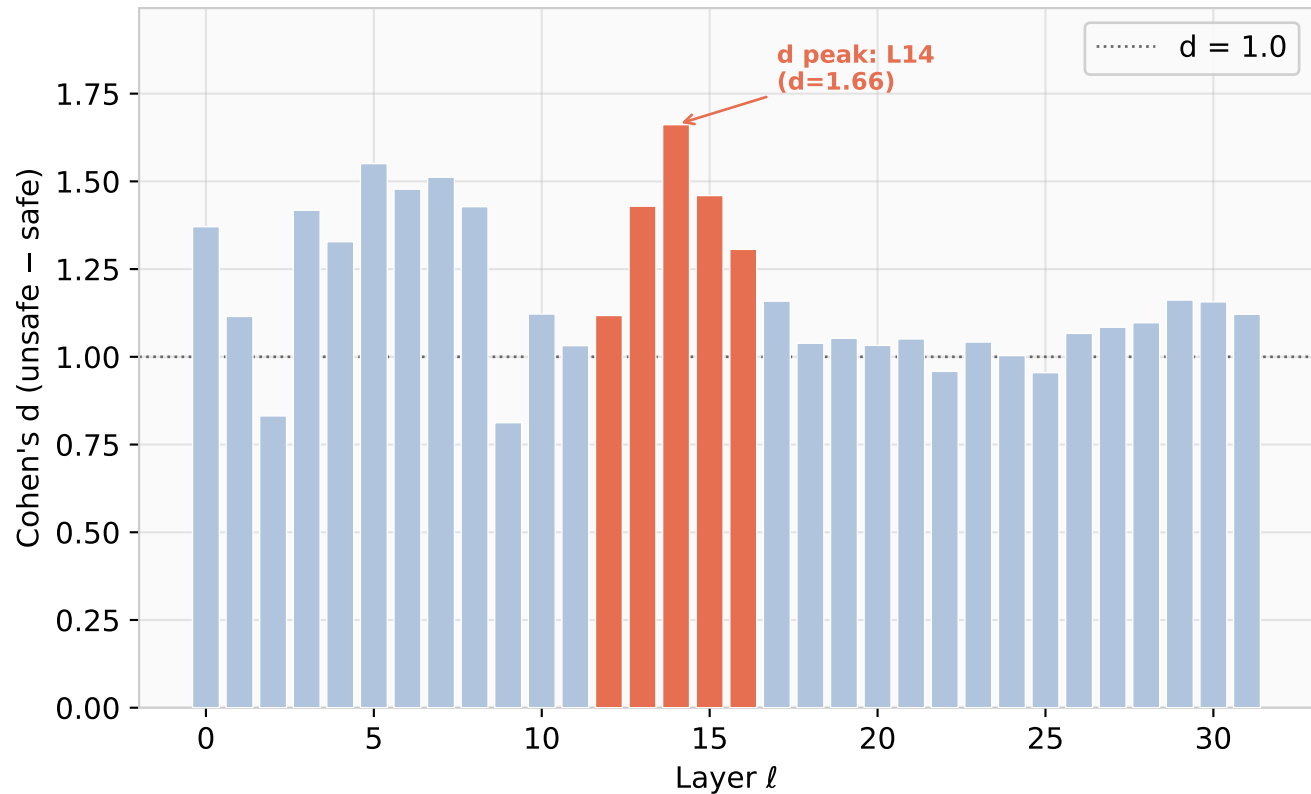
(b) Effect Size — d peaks at L14, \theta gap peaks at L17
