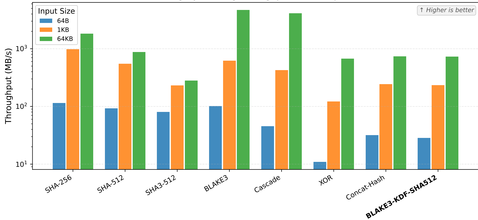
Data Integrity Hashing Throughput Across Input Sizes
