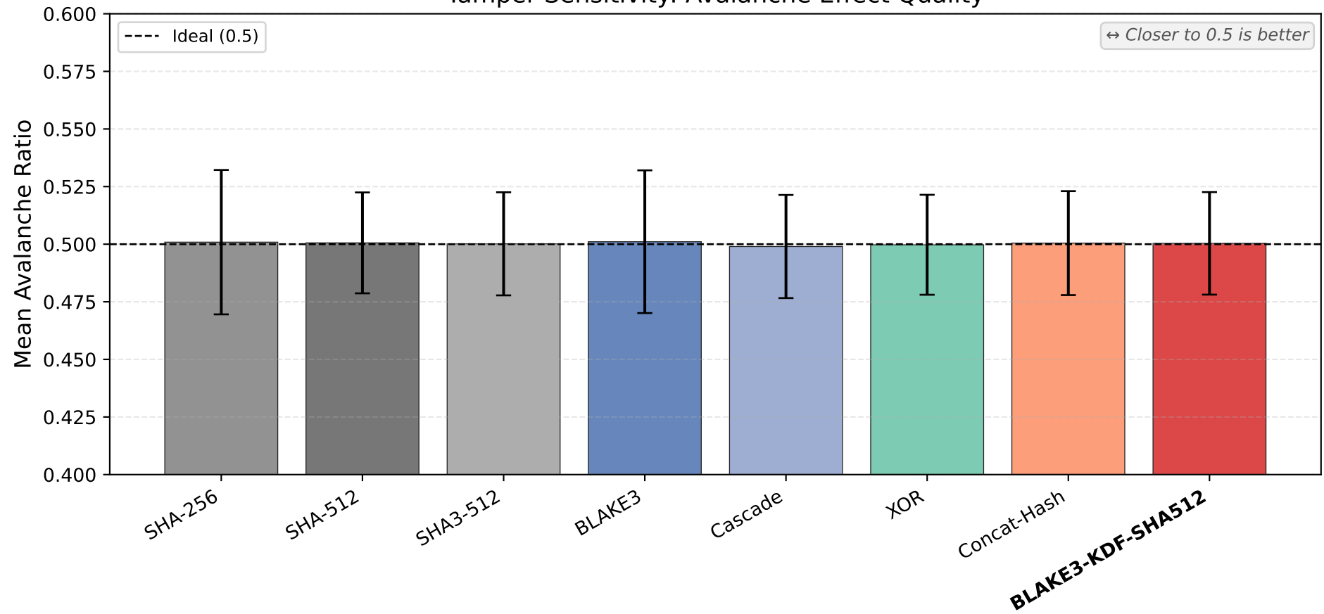
Tamper Sensitivity: Avalanche Effect Quality
