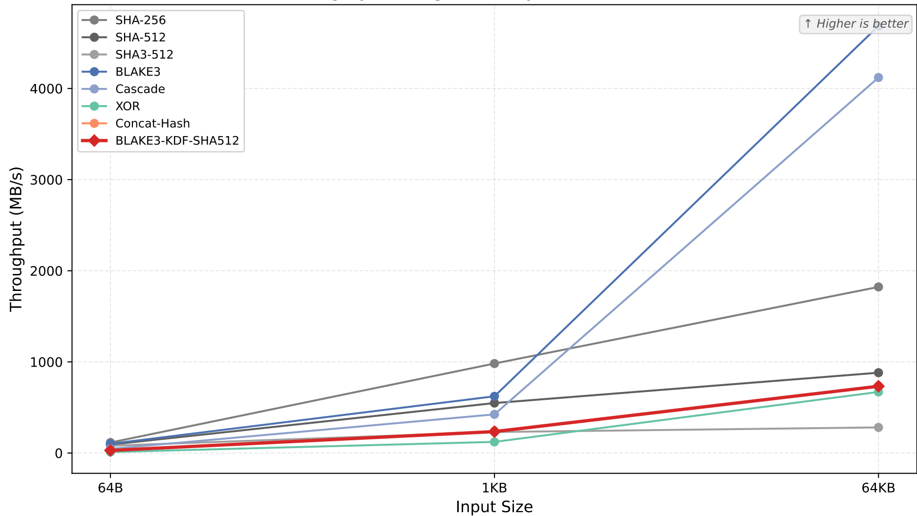
Integrity Hashing Scalability Across Data Sizes
