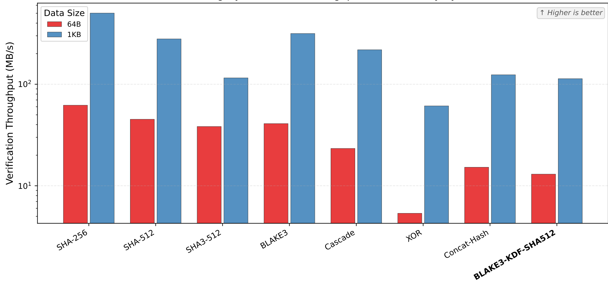
Data Integrity Verification Throughput (Hash + Verify Cycle)
