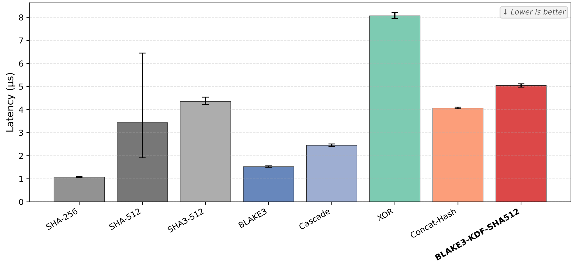
Integrity Hash Latency at 1KB Input (95% CI)
