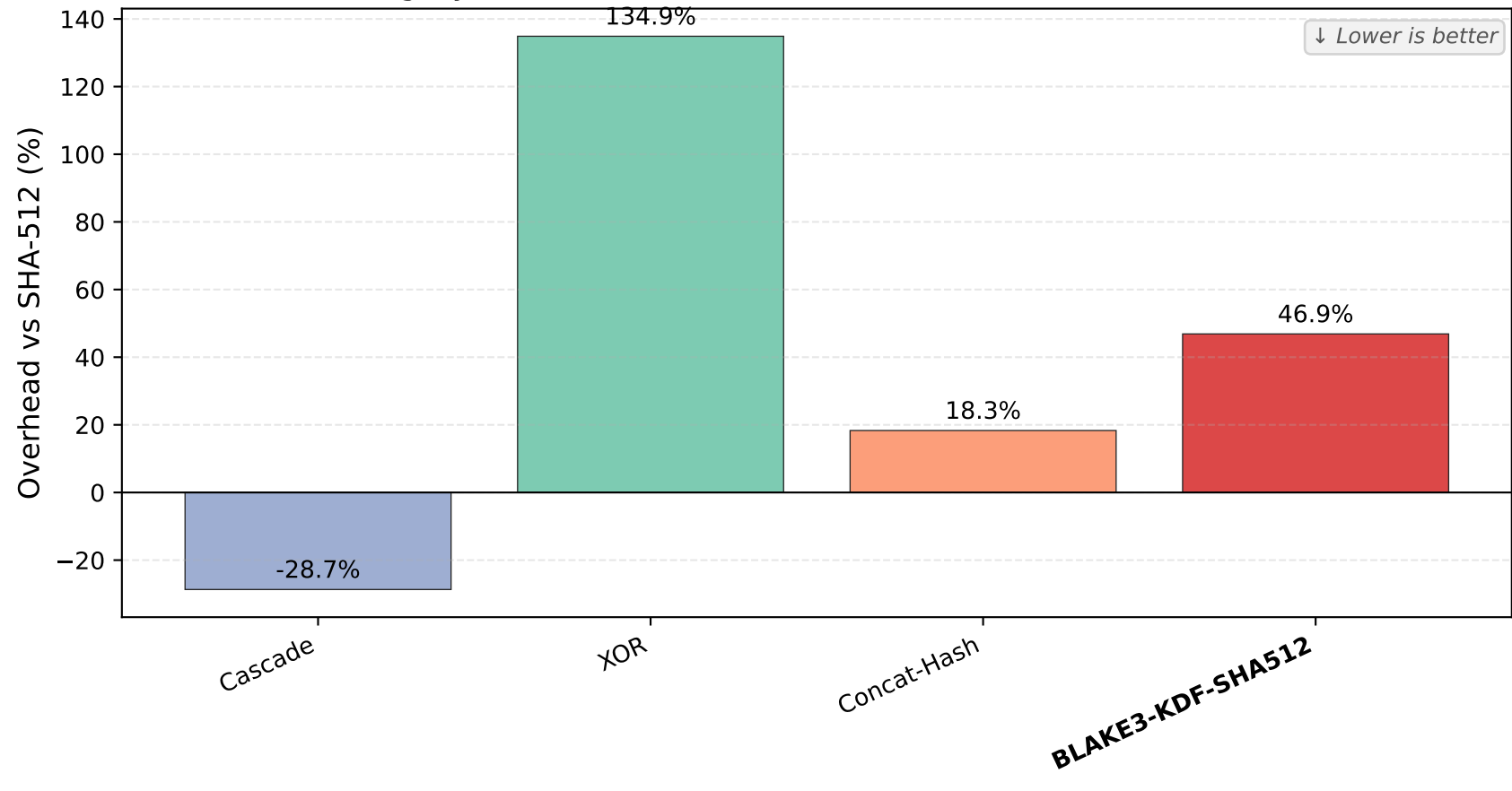
Integrity Framework Overhead vs Standalone SHA-512 (1 KB)
