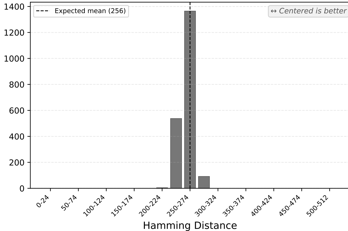
SHA-512
