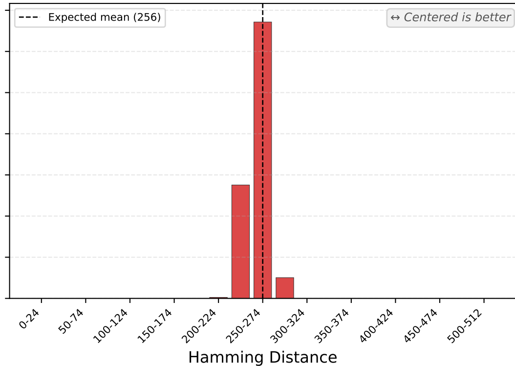
BLAKE3-KDF-SHA512
