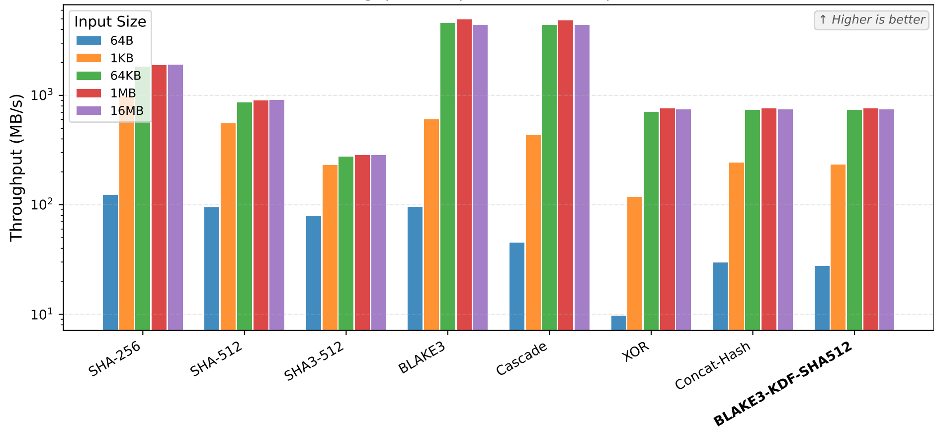
Throughput Comparison Across Input Sizes
