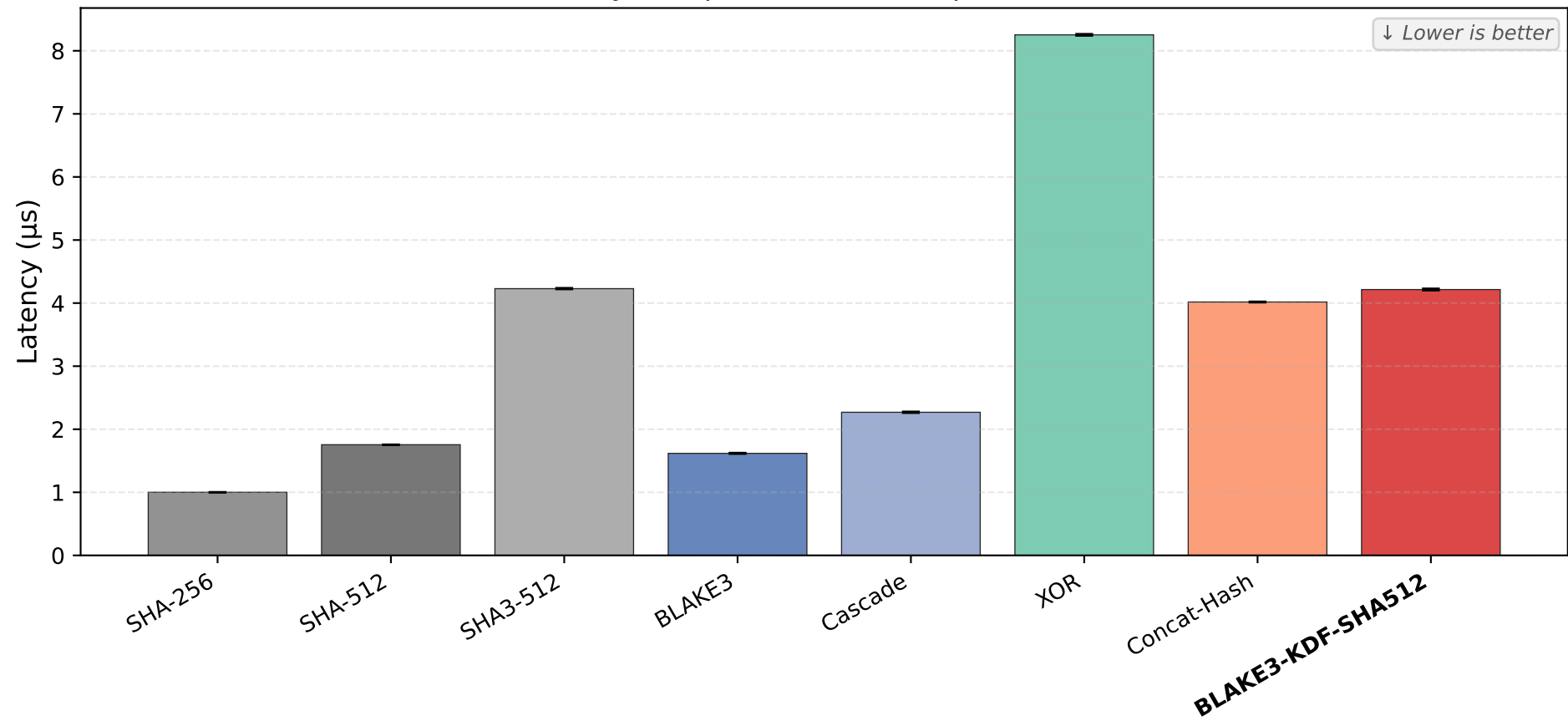
Latency Comparison at 1KB Input (95% CI)
