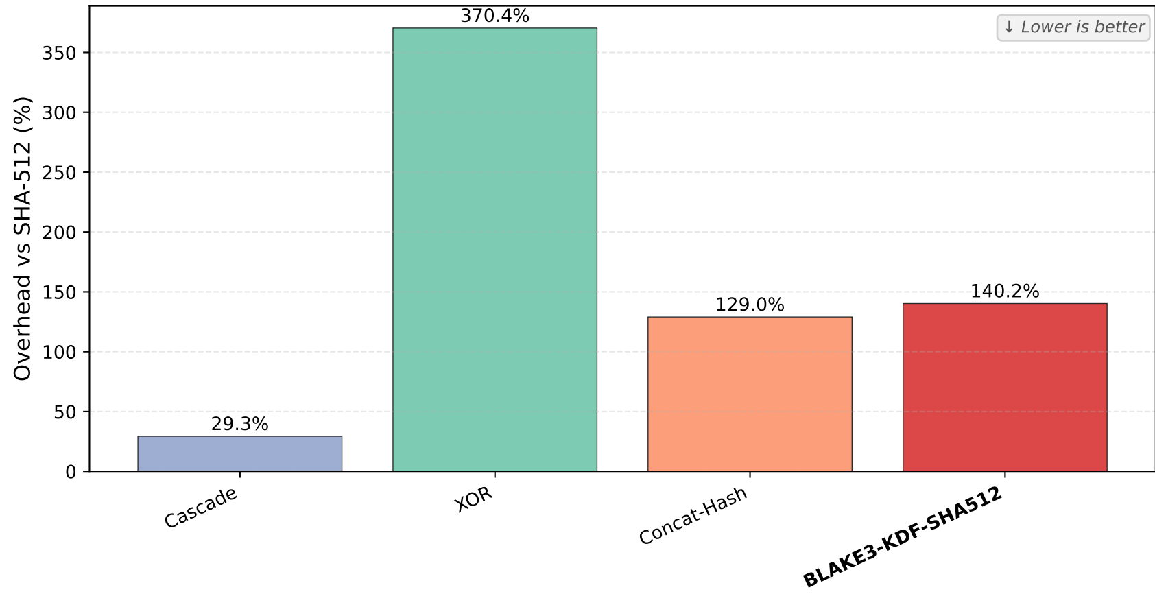
Combiner Latency Overhead at 1 KB Input
