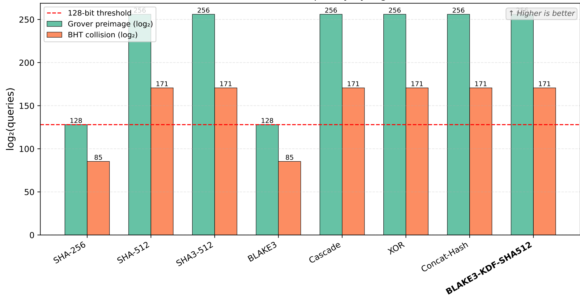
Quantum Attack Complexity by Algorithm
