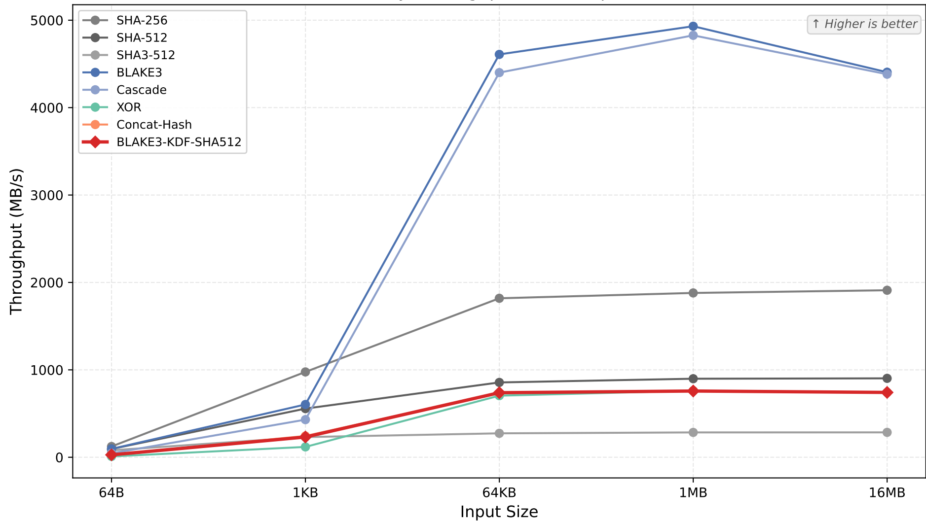
Scalability: Throughput Across Input Sizes
