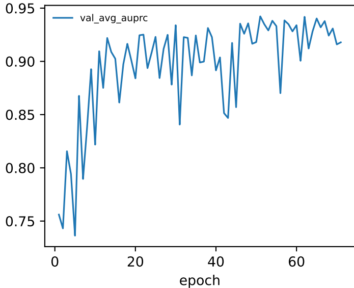
validation metric
