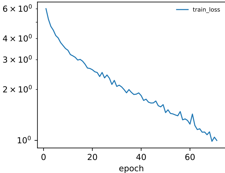
training loss
