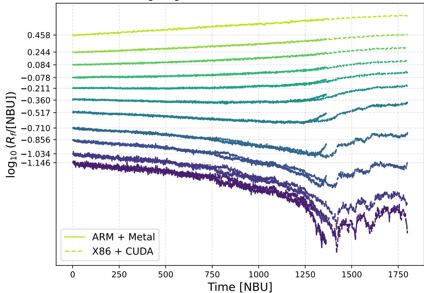
Lagrangian Radii Evolution (NBODY7)
