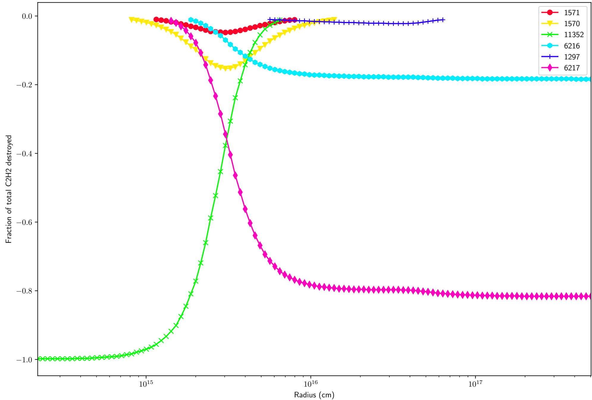
destruction-major-1-C2H2-model-2025-10-15h16-13-56
