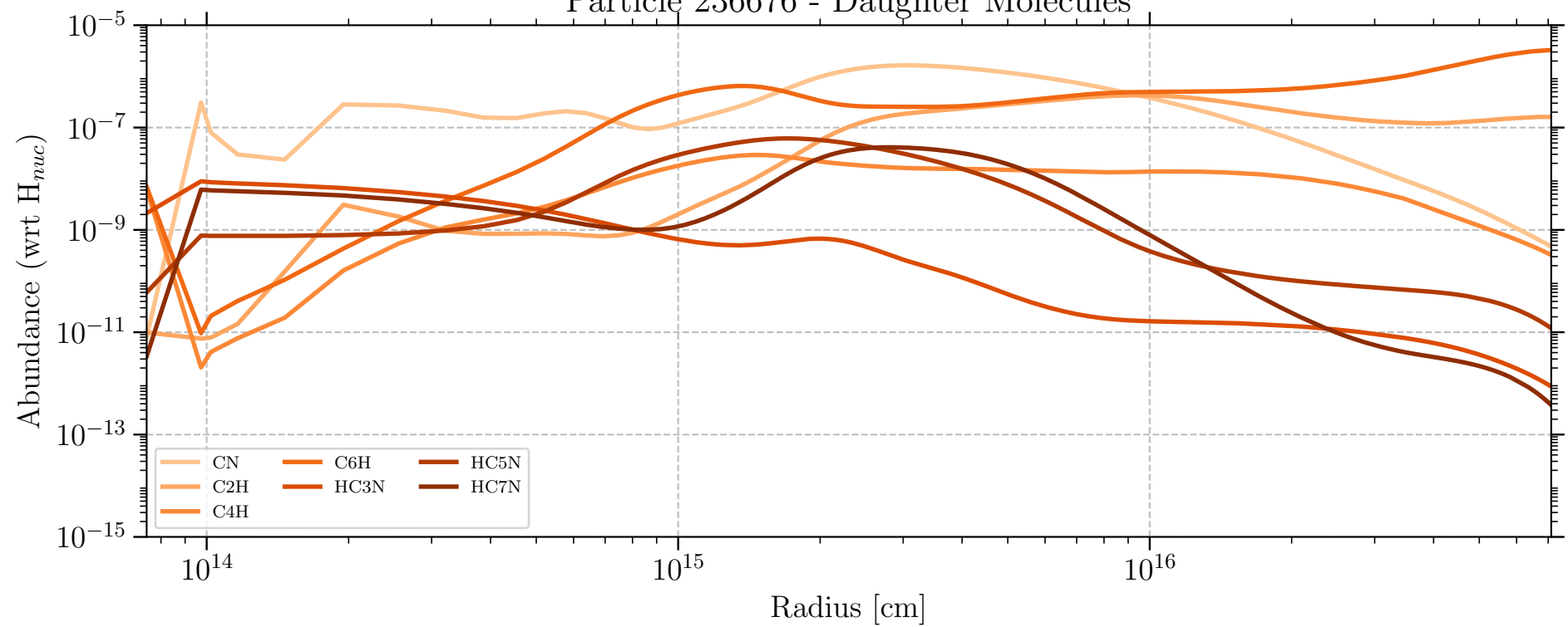
Particle 236676 - Daughter Molecules
