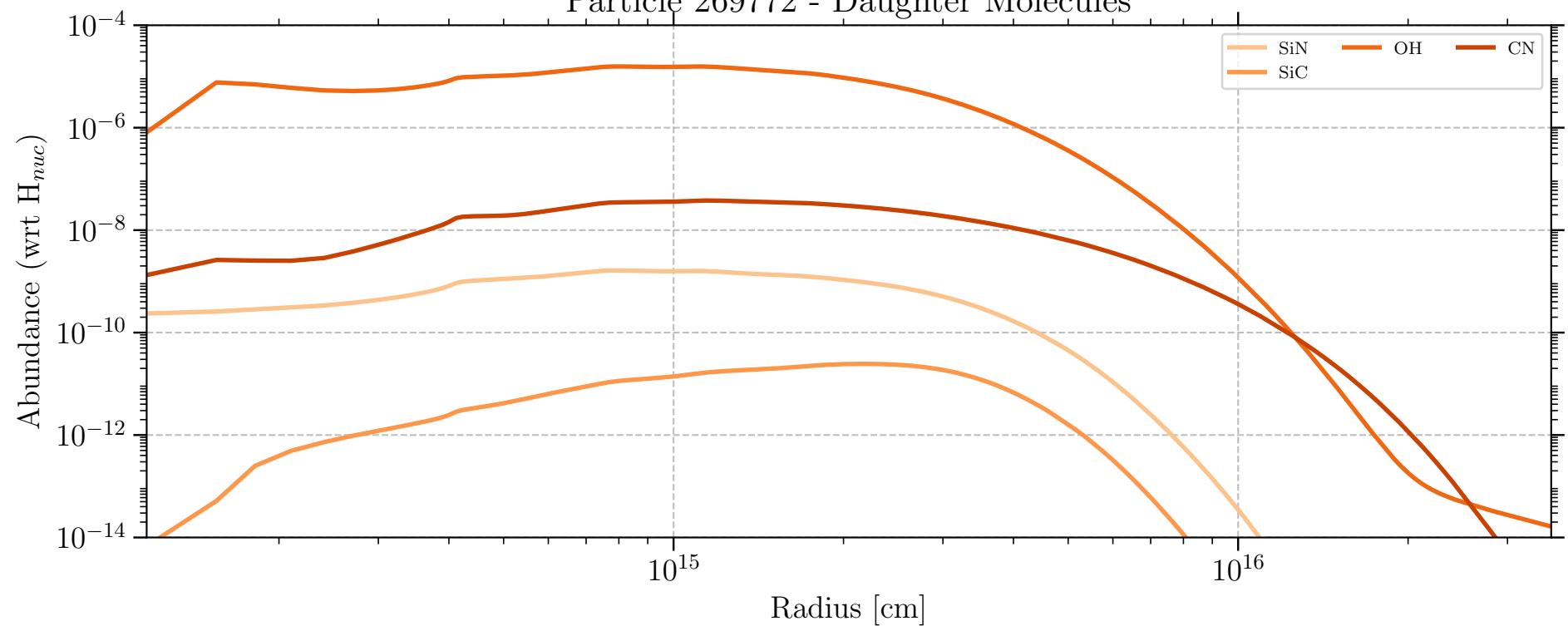
Particle 269772 - Daughter Molecules
