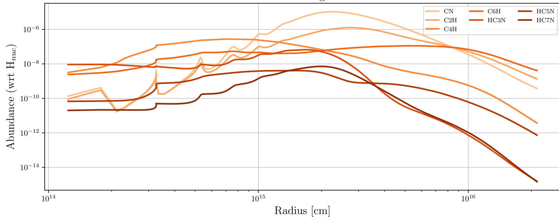
Particle 120838 - Daughter Molecules
