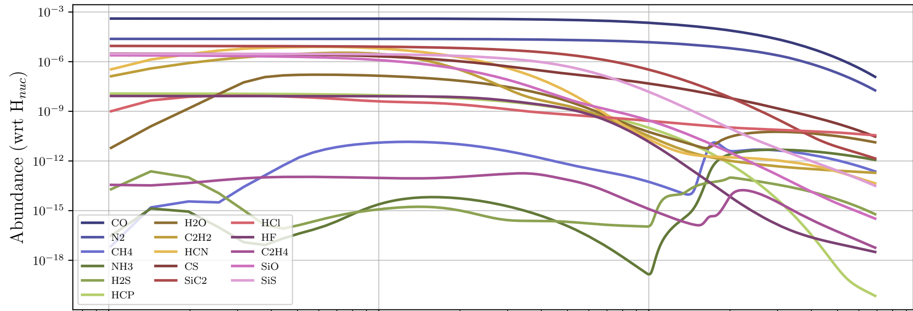
Particle 29823 - Daughter Molecules
