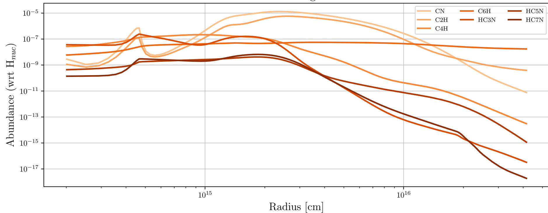
Particle 46371 - Daughter Molecules
