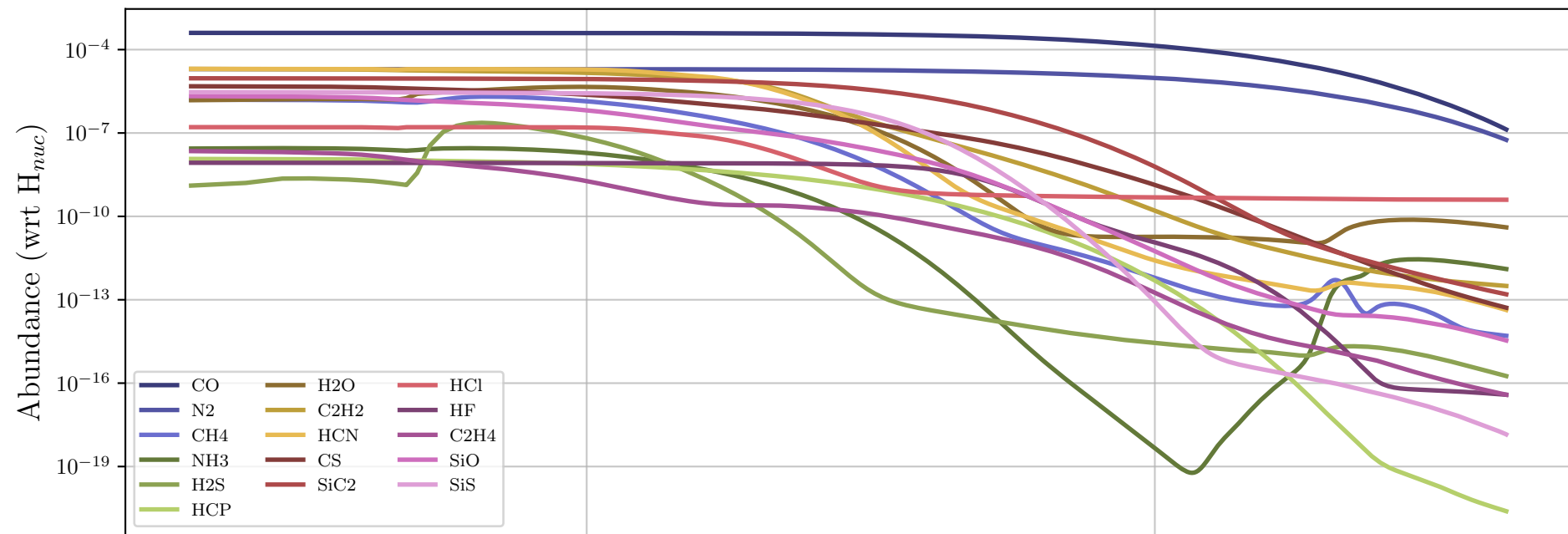
Particle 46371- Parent Molecules
