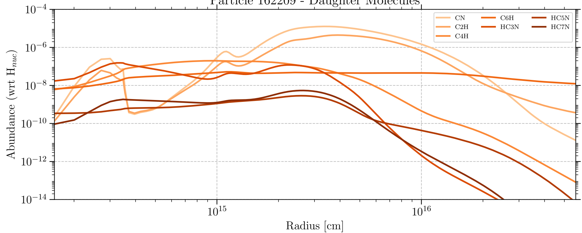
Particle 162209 - Daughter Molecules
