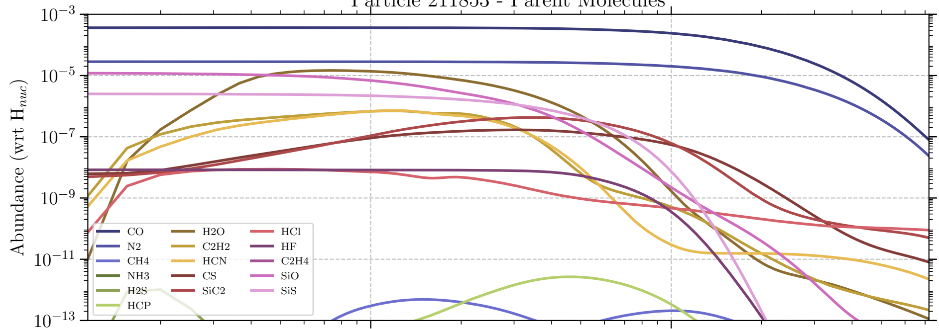
Particle 211853 - Daughter Molecules
