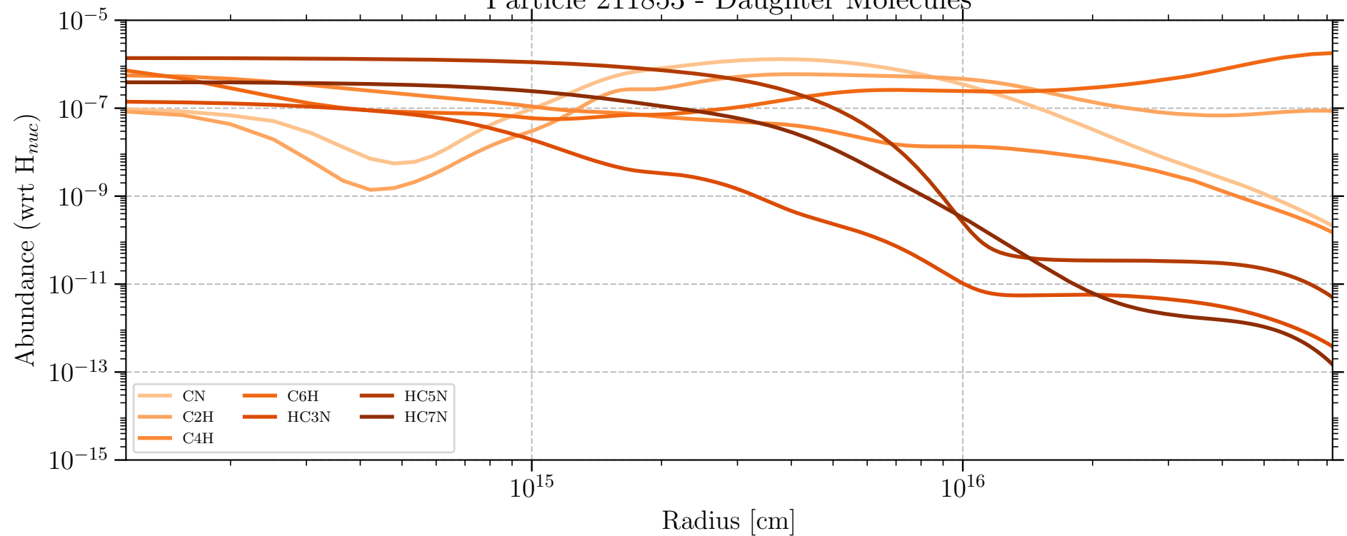
Particle 211853 - Daughter Molecules
