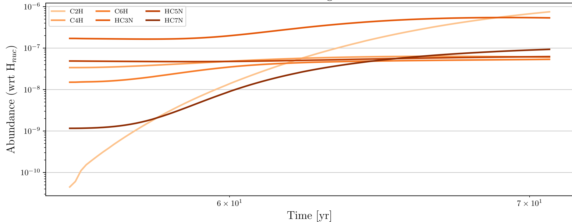
Particle 101515 - Daughter Molecules
