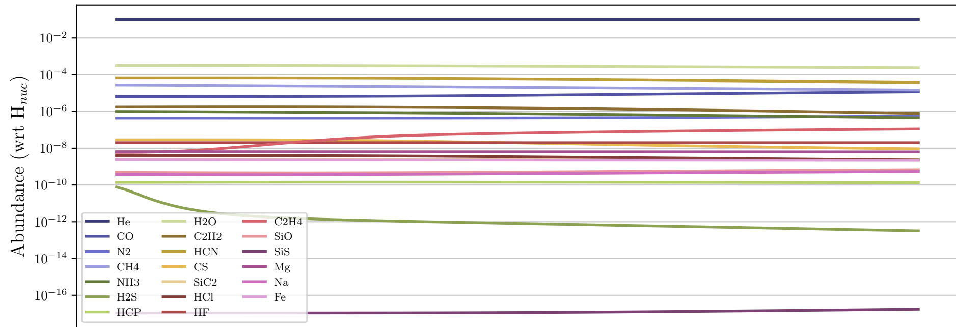
Particle 101515 - Parent Molecules
