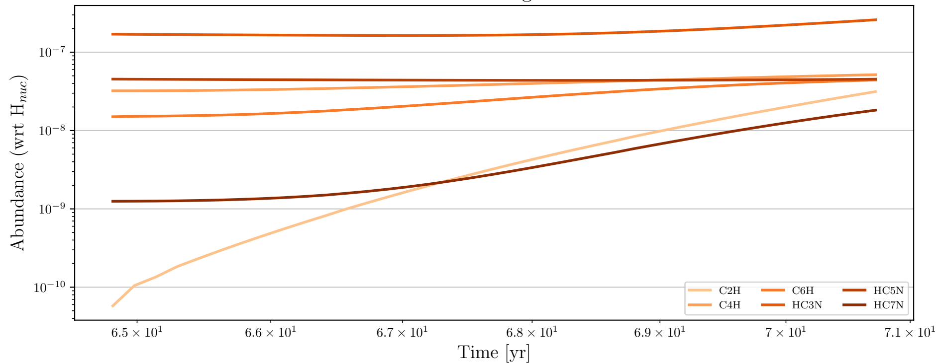
Particle 119063 - Daughter Molecules
