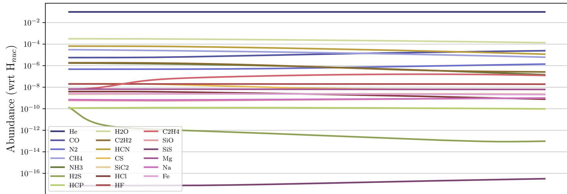
Particle 57645 - Daughter Molecules
