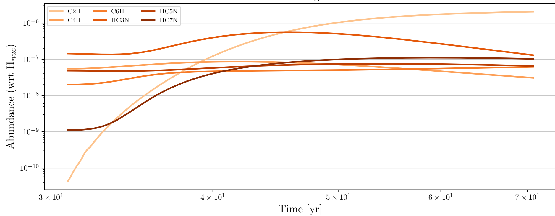
Particle 57645 - Daughter Molecules
