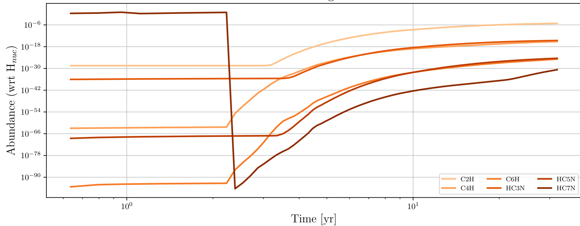
Particle 14806 - Daughter Molecules
