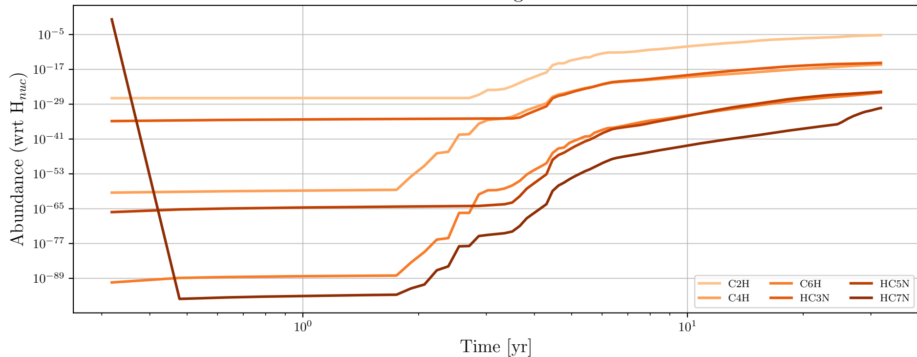
Particle 9203 - Daughter Molecules
