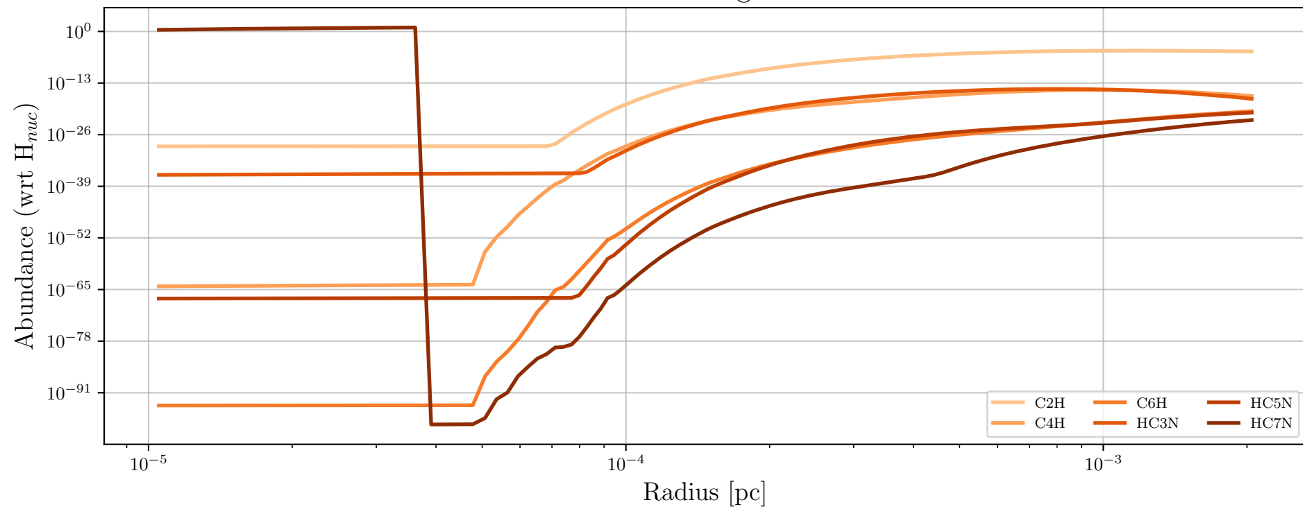
Particle 24631 - Daughter Molecules
