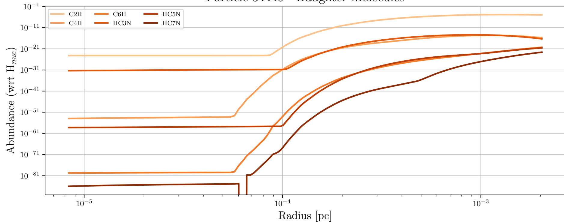
Particle 34446 - Daughter Molecules
