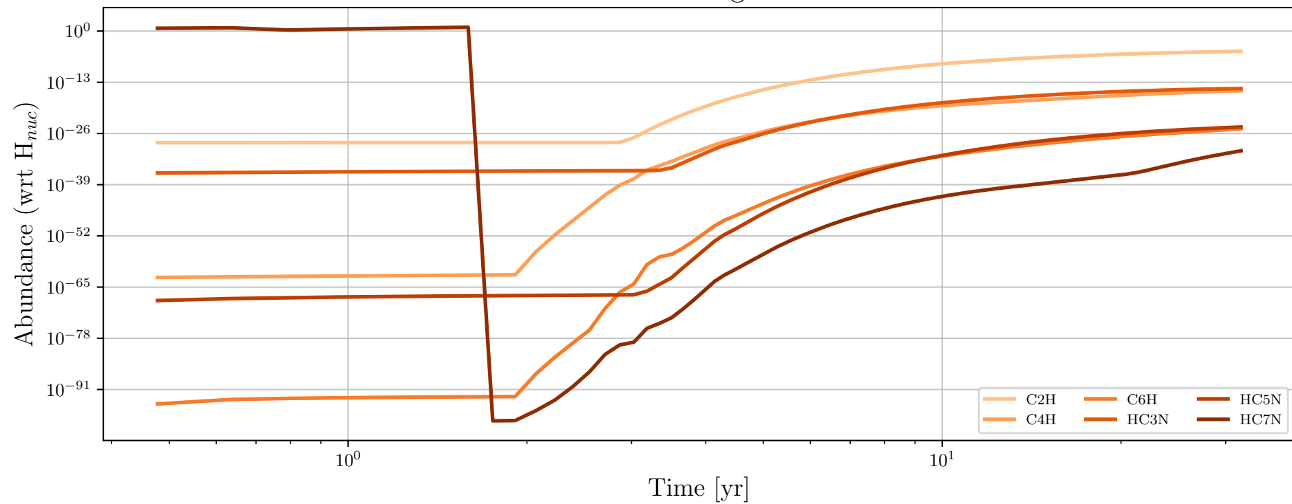
Particle 12005 - Daughter Molecules
