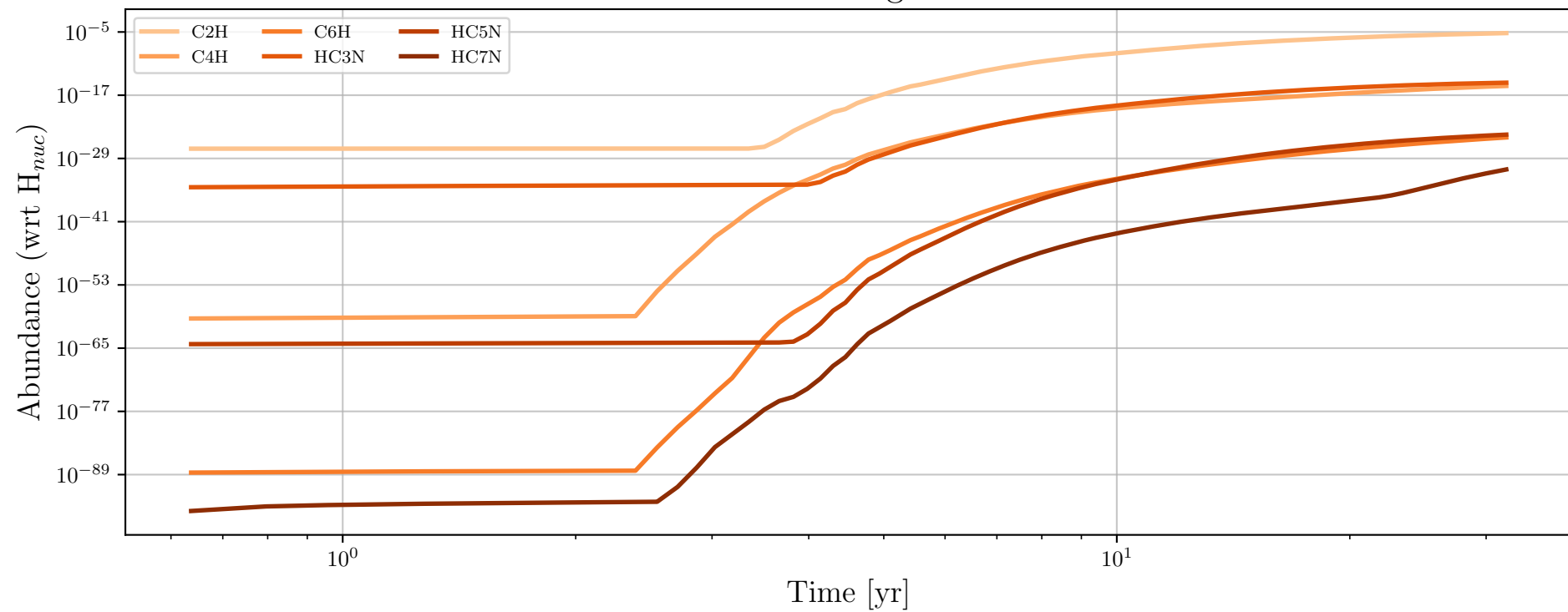
Particle 16207 - Daughter Molecules
