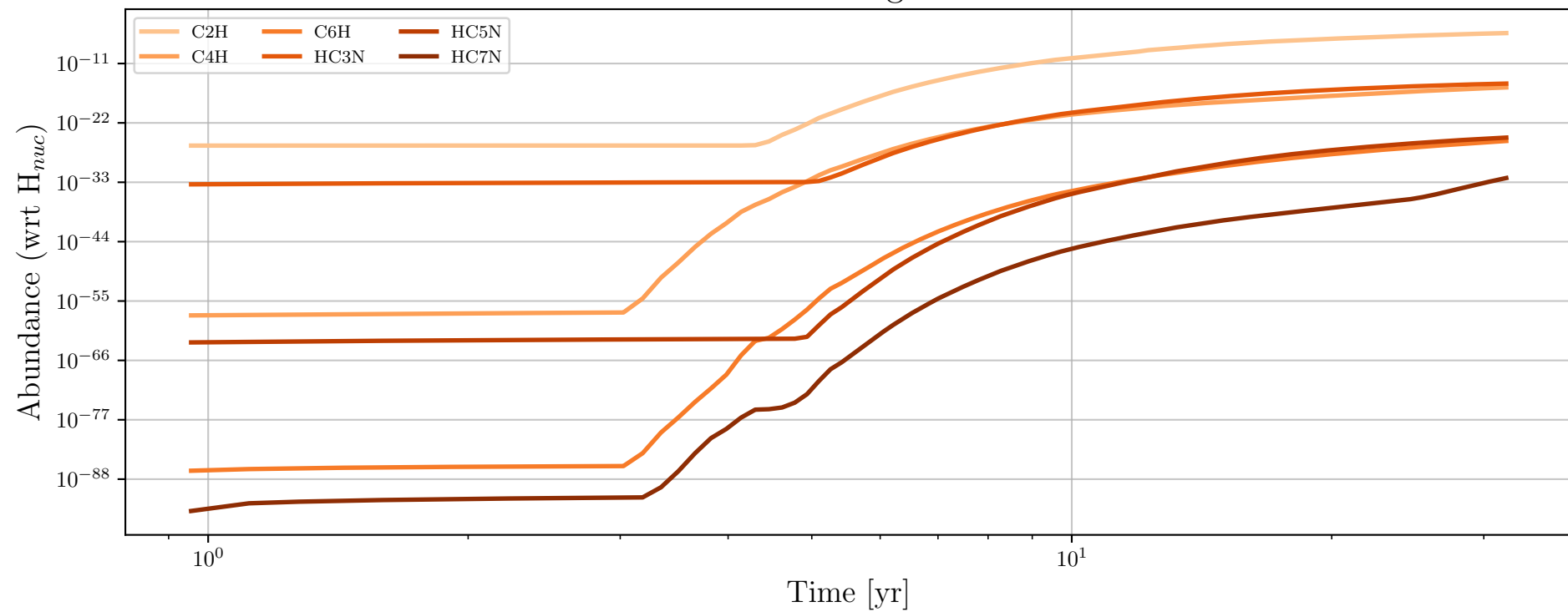
Particle 23211 - Daughter Molecules
